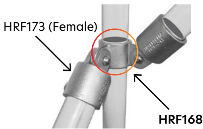
90° CORNER SWIVEL COMBINATION
