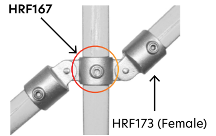
DOUBLE SWIVEL COMBINATION
